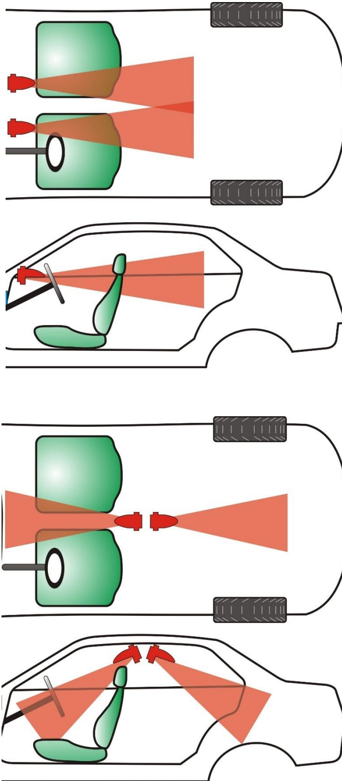
Figure 5 - Cockpit Nozzle Location/Orientation
