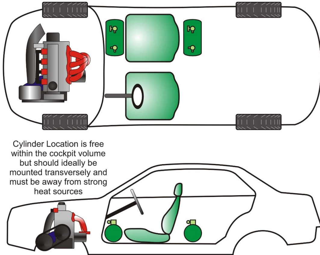
Figure 6 – Extinguisher Location
