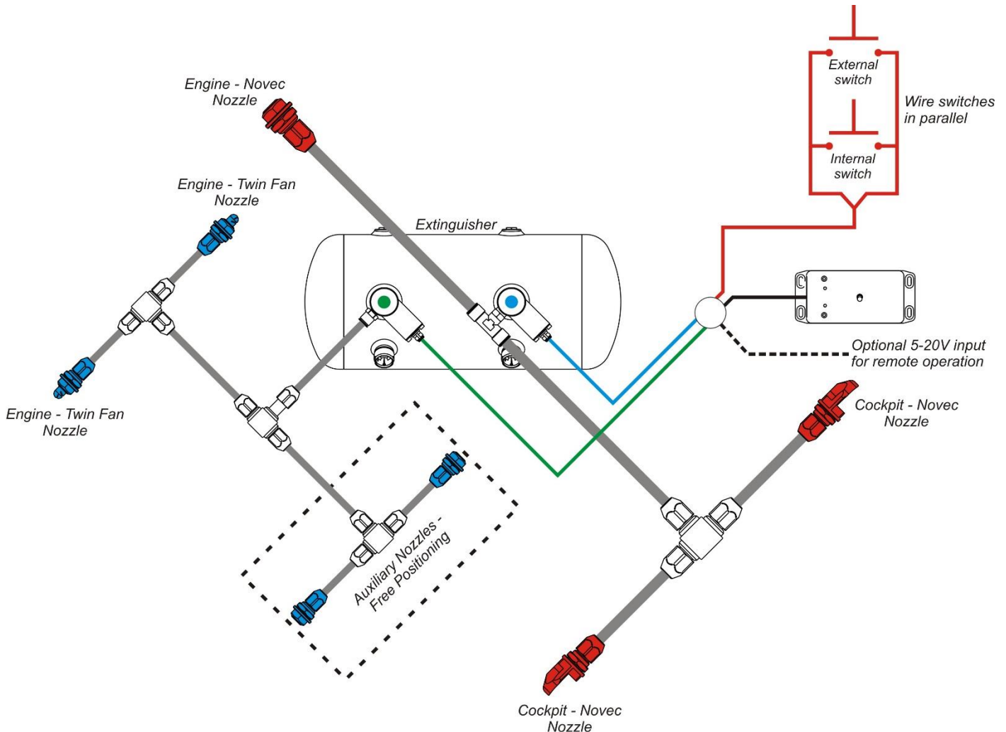
Figure 7 – System Schematic
