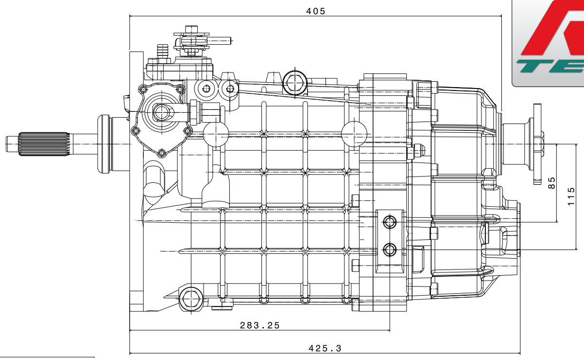
Gearbox SCL90-20
