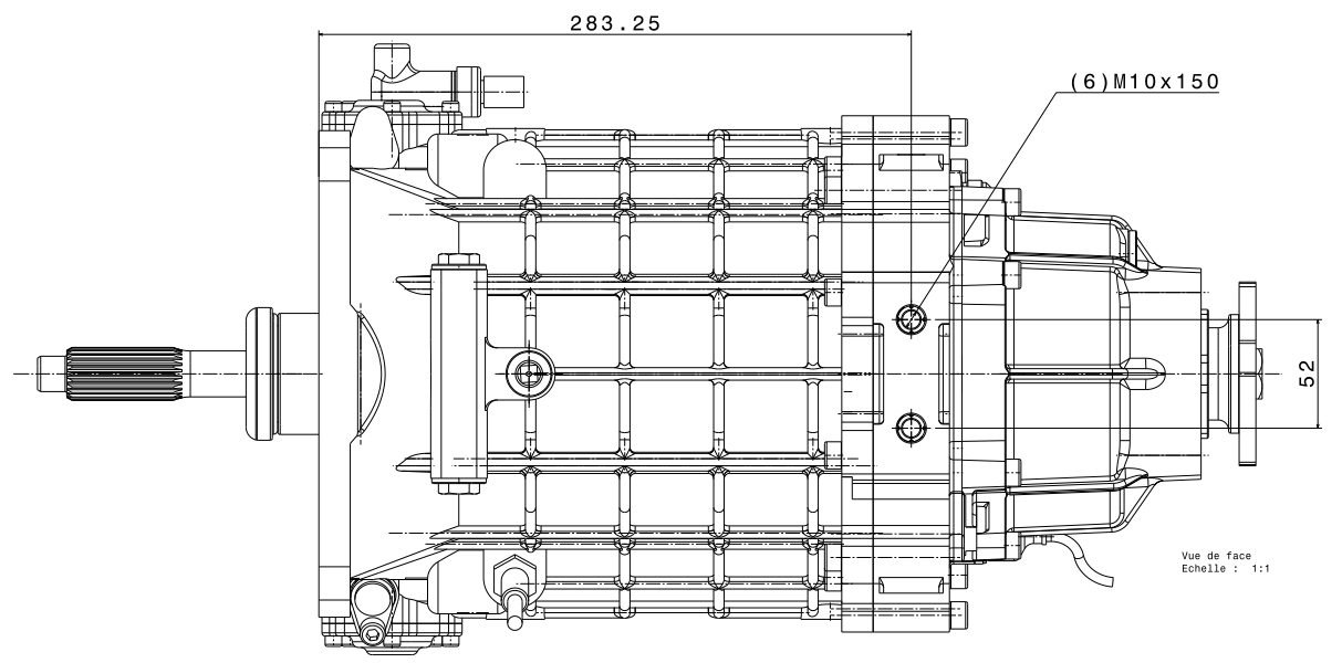
Gearbox SCL90-20
